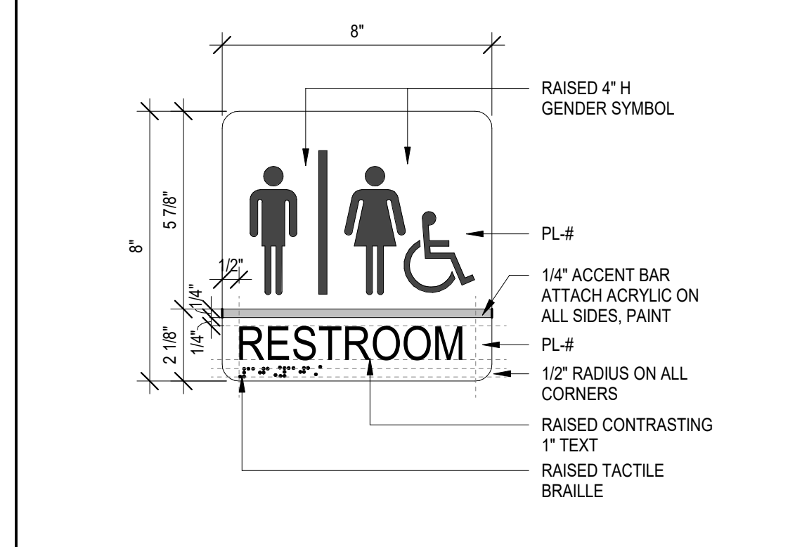
24 SIGN R 3" = 1'-0"
