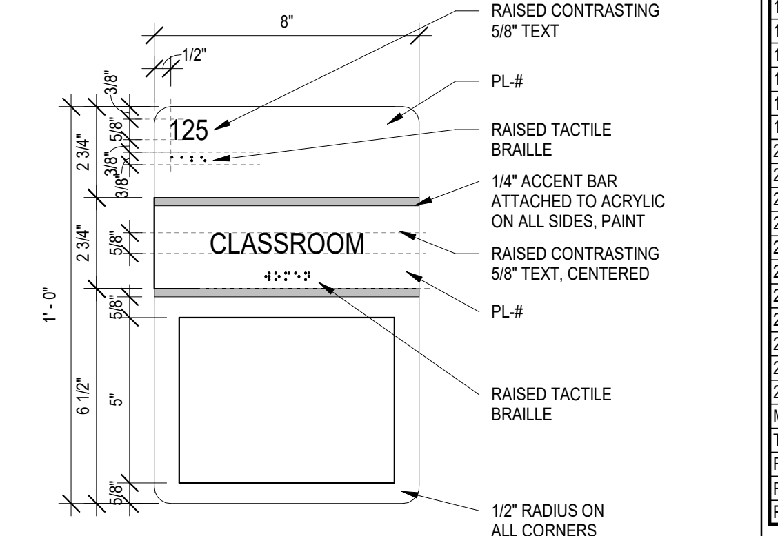
20 SIGN C 3" = 1'-0"
