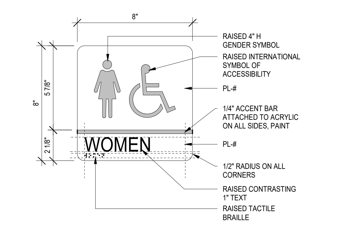
22 SIGN W 3" = 1'-0"
