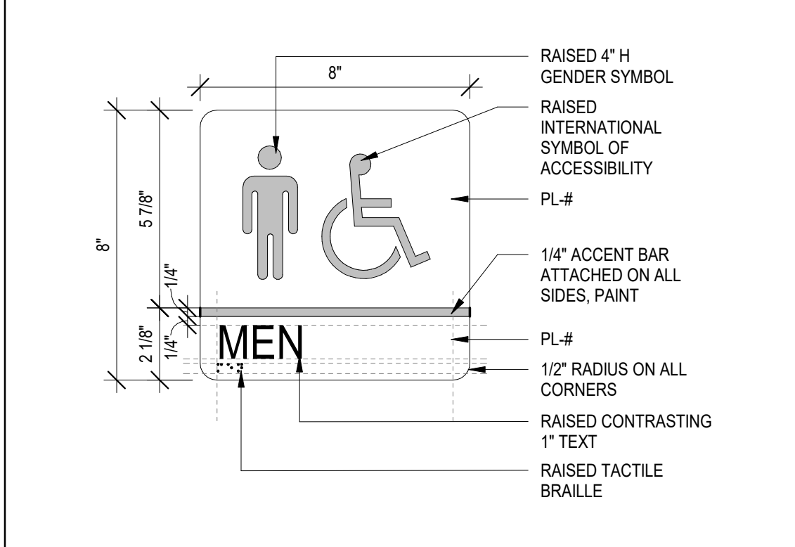
23 SIGN M 3" = 1'-0"
