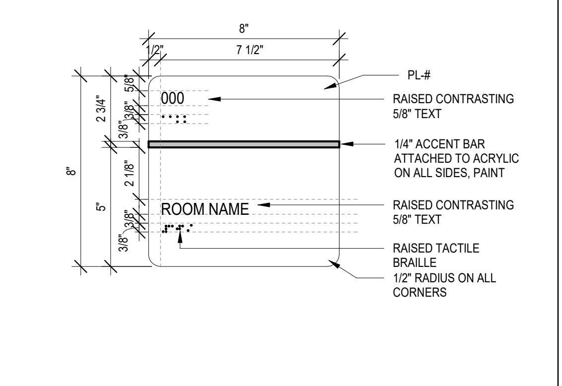
21 SIGN J 3" = 1'-0"
